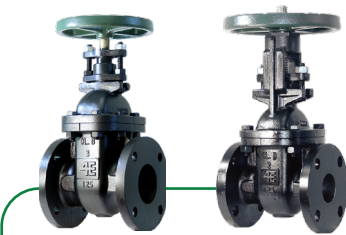
OS&Y AND NRS GATE VALVE
