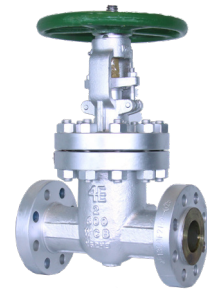
GATE VALVE (OS&Y, NRS)
