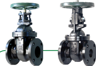
OS&Y AND NRS GATE VALVE Cast Iron | 2"- 36" | 125#
